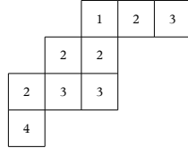
Fig. 3: A semistandard skew tableau of shape (5, 3, 3, 1)/(2, 1) and type (1, 4, 3, 1) . Its reverse reading word is (3, 2, 1, 2, 2, 3, 3, 2, 4) , which is not a lattice permutation, but an \alpha -lattice permutation for \alpha = (4, 1) .
