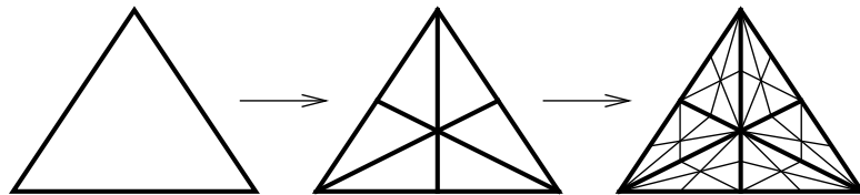
FIGURE 8. Barycentric subdivision in a 2-simplex, iterated twice.
