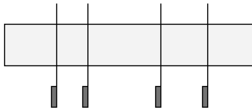
FIGURE 6. A cut-set of a cake.
