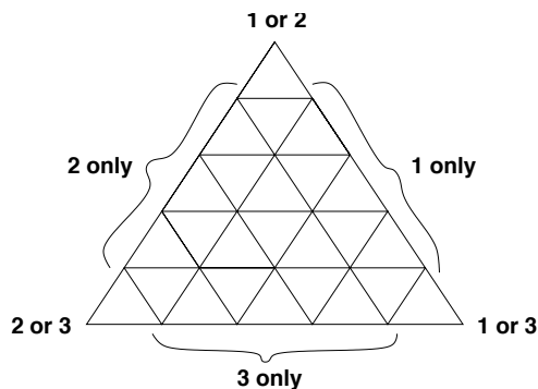
FIGURE 9. The dual labelling arising from rent-partitioning.
