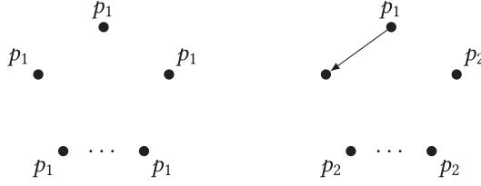
Fig. 5. Impartial probability assignment for two graphs with n vertices.
