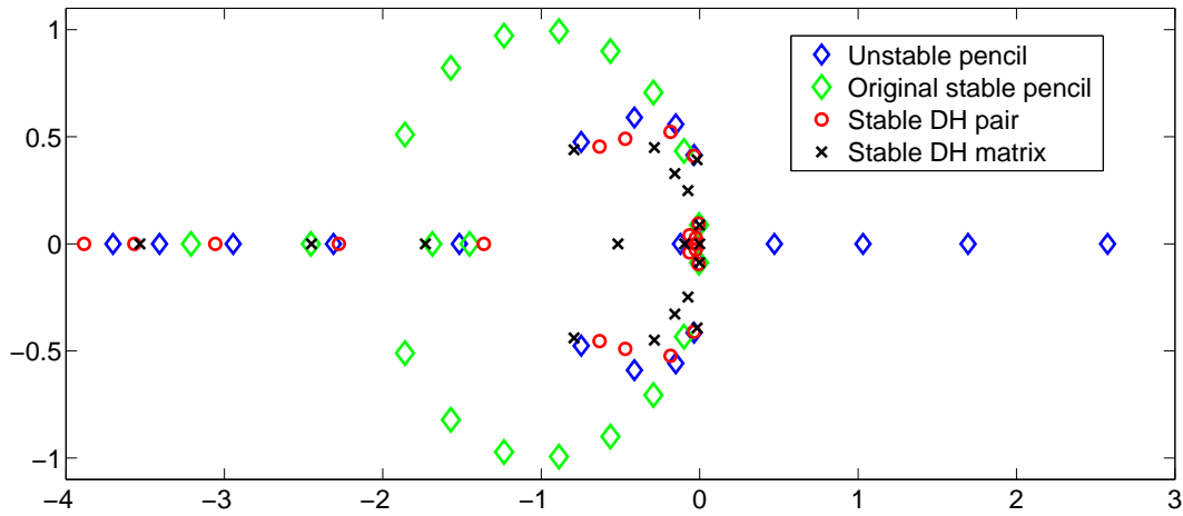
Figure 5.4: Eigenvalues of various pencils corresponding to the mass-spring-damper system.
