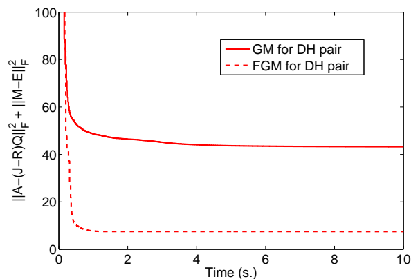
Figure 5.2: Evolution of the objective function for the different algorithms for matrix pair (E, A) where A is Gaussian and E is the best rank- r approximation of a Gaussian matrix, n = 20 and r = 3 .
