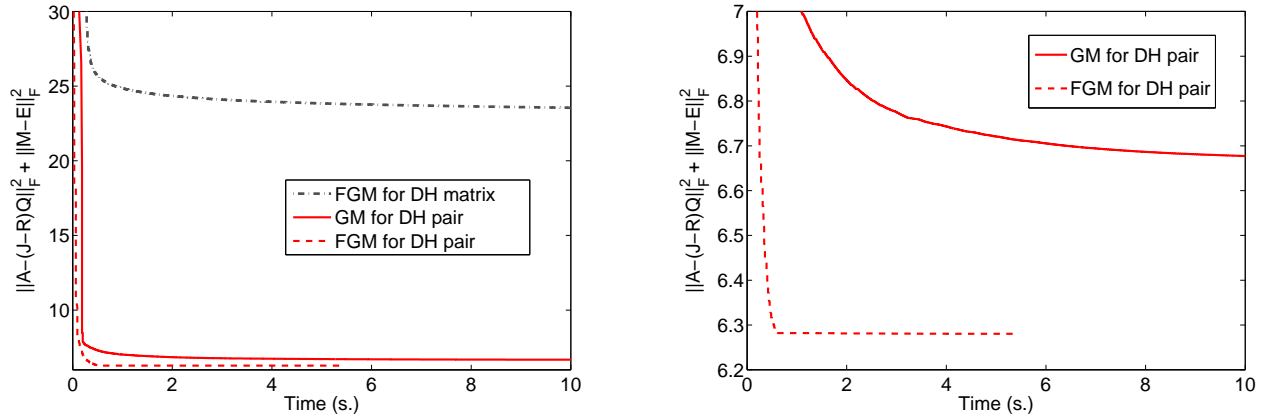
Figure 5.1: Evolution of the objective function for FGM and GM for the matrix pair (I_n, A) where A is a 20 \times 20 Grcar matrix of order 3. The right figure is a zoom of the left figure and shows the fast convergence of FGM compared to GM.
