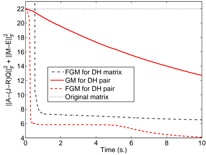
Figure 5.3: Evolution of the objective function for the different algorithms for matrix pair (E, A) for the perturbed mass-spring-damper system.
